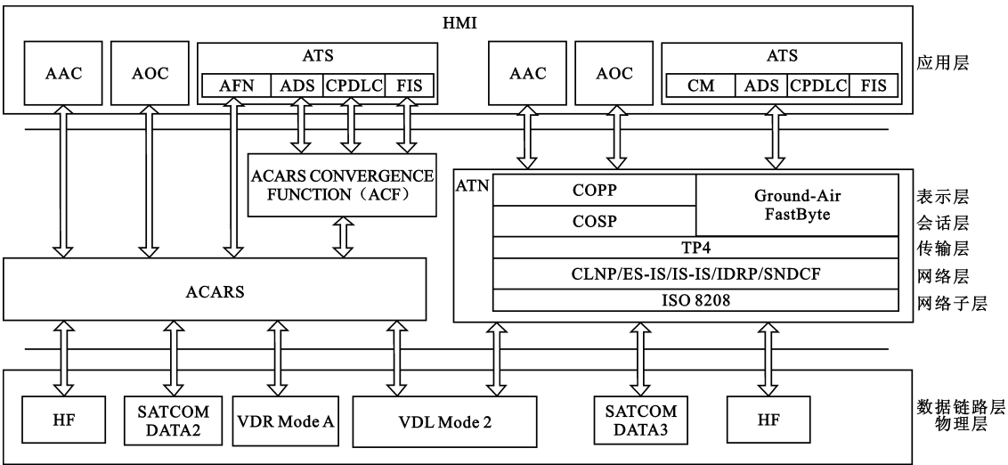
图 4 通信管理 ACARS 和 ATN 双协议栈 Fig.4 ACARS and ATN dual protocol stack of communication management
